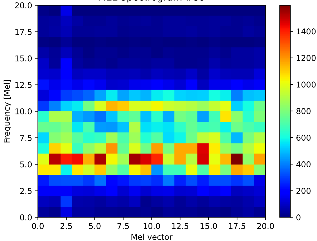
MEL Spectrogram #39
